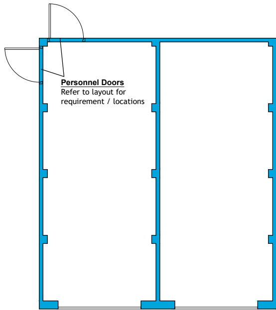
Floor Plan DG2 (Single Garages)
